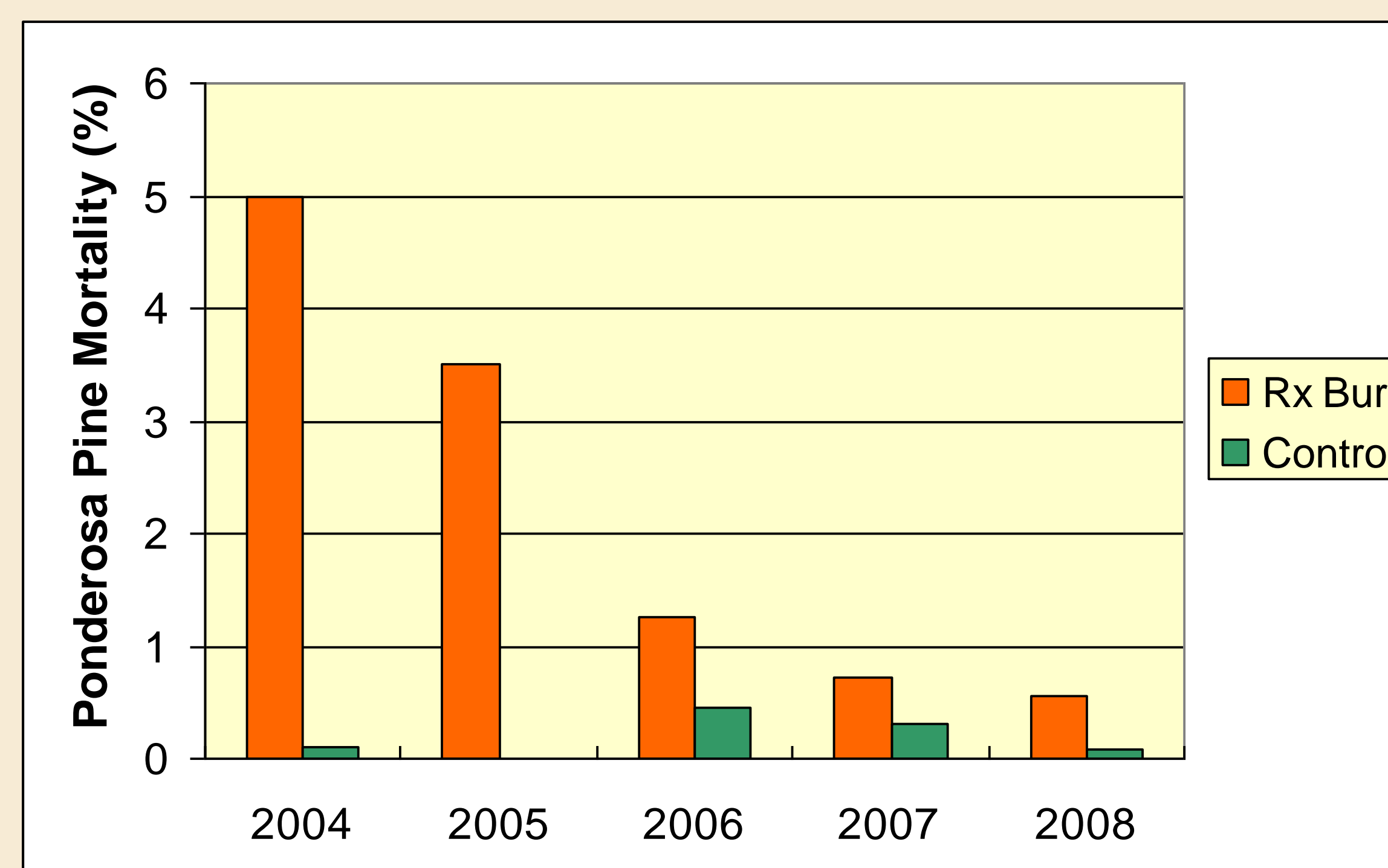
Figure 1. Annual bark beetle-induced ponderosa mortality found at sites in Arizona and New Mexico
